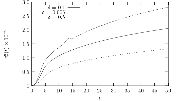
Fig. 12. Maximal value of the generated fast magnetoacoustic wave, V_x^a(t) , versus time. Solid, long dashed and short dashed curves represent solutions of Eq. (12) using 2D MacCormak code on 4000 \times 4000 spatial resolution for \delta = 0.1, 0.005, 0.5 accordingly.
