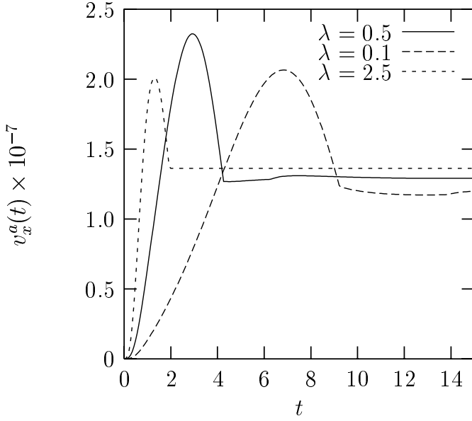
Fig. 9. Maximal value of the generated fast magnetoacoustic wave, V_x^a(t) , versus time. Solid, long dashed and short dashed curves represent solutions of Eq. (16) using 1D MacCormak code on 20 000 spatial resolution for \lambda = 0.5, 0.1, 2.5 accordingly.
