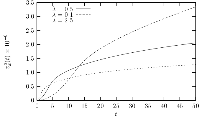
Fig. 11. Maximal value of the generated fast magnetoacoustic wave, V_x^a(t) , versus time. Solid, long dashed and short dashed curves represent solutions of Eq. (12) using 2D MacCormak code on 4000 \times 4000 spatial resolution for \lambda = 0.5, 0.1, 2.5 accordingly.
