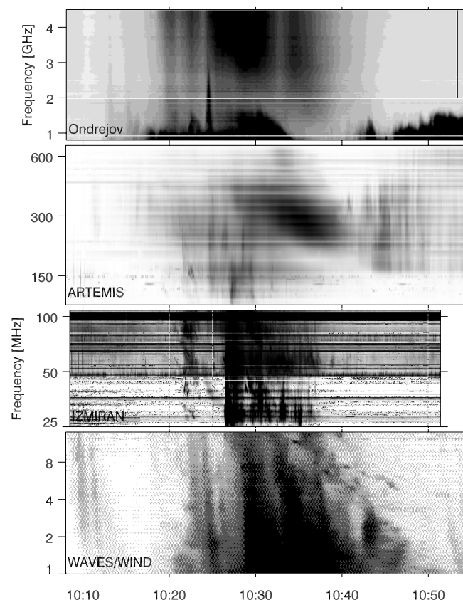
Fig. 2. Radio spectra from microwaves to hectometric waves during the 14 July 2000 event. From top to bottom: Ondřejov Observatory (Karlický et al. 2001), Artemis-IV, Thermopylae, Greece (courtesy C. Alissandrakis; Caroubalos et al. 2001), IZMIRAN, WAVES/Wind (courtesy M. Kaiser). Dark shading means bright emission.
