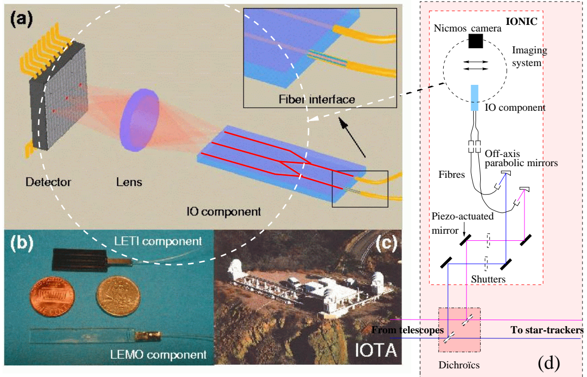
Fig. 1. a) Optical layout of the experiment (credits: E. Stadler). The LEMO chip's three outputs (described in the text) are imaged onto a liquid nitrogen cooled infrared detector matrix. b) Integrated optics components, top: LETI beam combiner, bottom LEMO beam combiner. c) IOTA interferometer. d) Optical breadboard.
