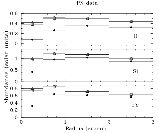
Fig. 3. PN profiles for O, Si and Fe. Symbols as in Fig. 2.
