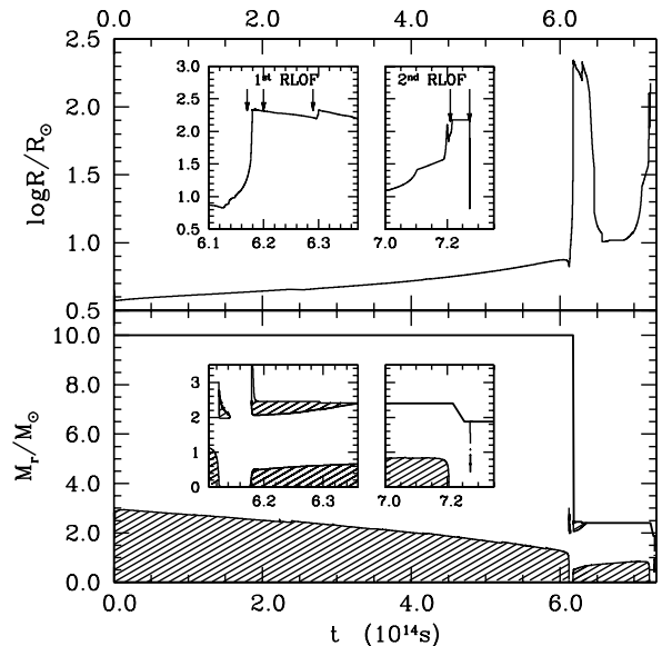
Fig. 3. Evolution of the main structure parameters as a function of time during the first and the second mass-loss episodes. The upper panel shows the evolution of the radius of the primary. The inserts show the mass-loss episodes with higher resolution. The lower panel shows the convective zones engendered during the evolution up to off-center ignition of carbon.
