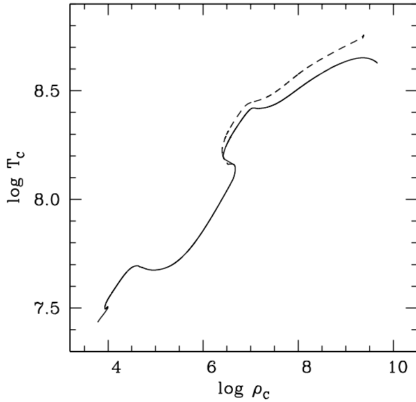
Fig. 7. Evolution in the \log \rho - \log T plane of the central layer of the isolated 10 M_\odot star (dashed line) and the of the primary component of the close binary system studied here (solid line), until the onset of carbon burning.
