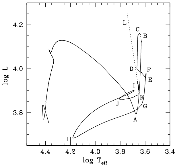
Fig. 2. Evolutionary track of the primary component in the Hertzsprung–Russell diagram. The physical quantities of the labeled models are shown in Table 1.
