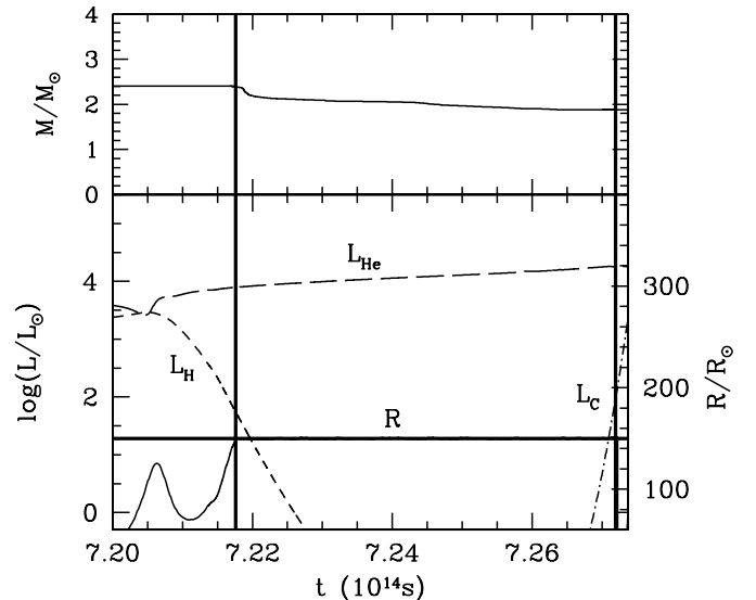
Fig. 6. Global characteristics of the primary component as a function of time during the second mass loss episode. The upper panel shows the total mass as a function of time. The lower panel shows the surface radius and the luminosities provided by hydrogen, helium and carbon burning. The vertical thin lines delimit the second mass loss episode. The surface luminosity is mostly provided by helium combustion.
