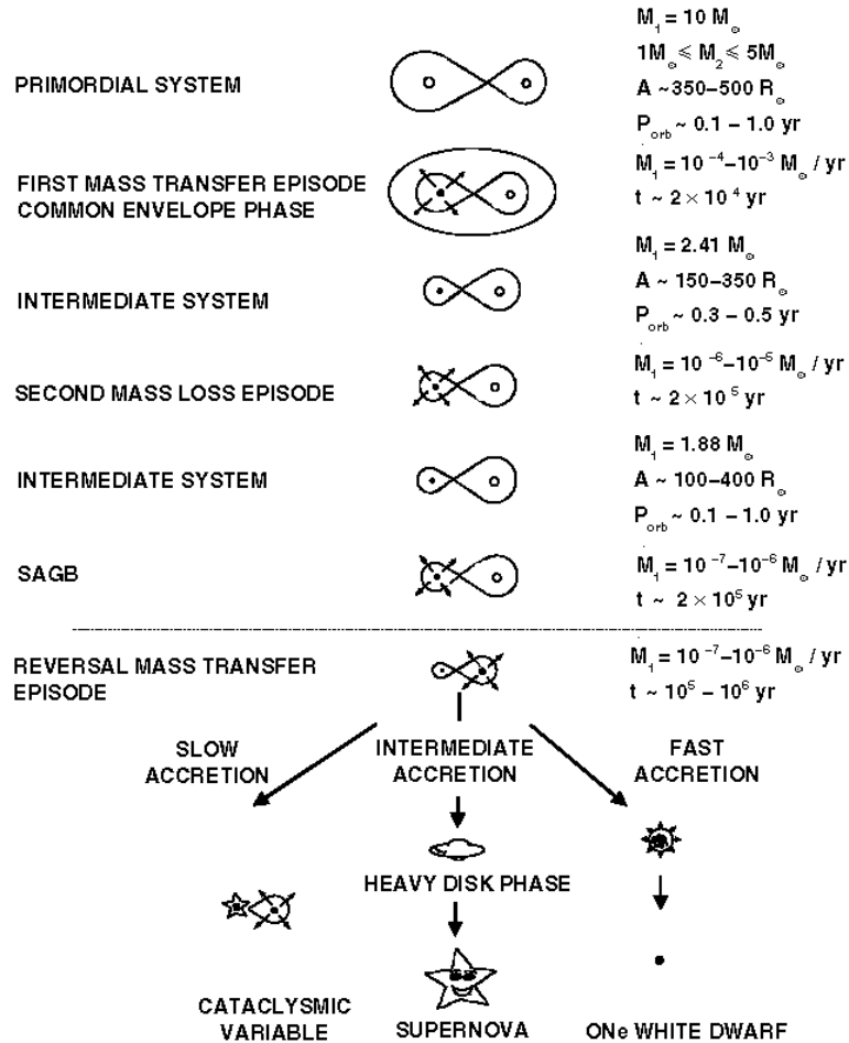
Fig. 1. Approximate evolution of the orbital parameters of the binary system and outline of the possible final outcomes. The dashed line divides the calculations reported in this paper and the three possible outcomes.
