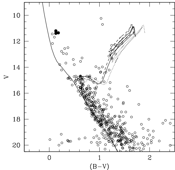
Fig. 7. CMD in the region of Loden 165. Superimposed are three solar metallicity isochrones for the ages of 2 (dotted line), 3 (solid line) and 4 (dashed line) Gyrs (Girardi et al 2000). The three filled circles indicate Lodén's triplet
