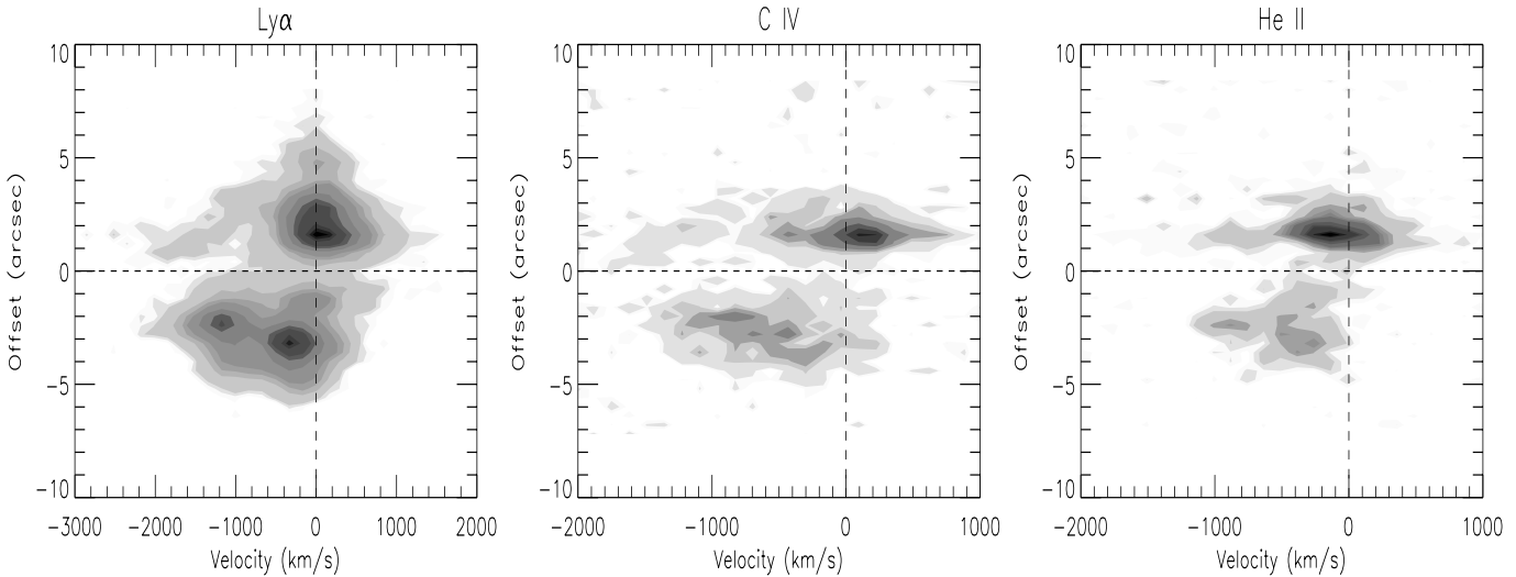
Fig. 3. The two-dimensional emission line structures of Ly \alpha , C IV and He II. Offset zero was chosen in between the northern and southern regions. Velocity zero corresponds to the peak Ly \alpha emission in the northern region
