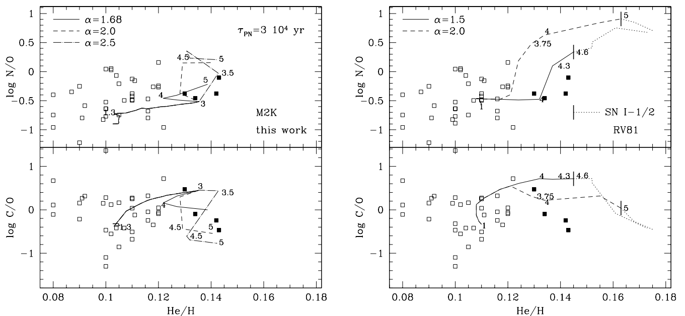
Fig. 11. Abundance ratios of galactic planetary nebulae. Observed data (squares) are taken from Kingsburgh & Barlow (1994), and Henry et al. (2000a). Filled squares correspond to PNe with \log(N/O) > -0.5 and He/H > 0.125 . Predicted PN abundances are shown as a function of the initial mass of solar-metallicity progenitor stars, as derived in this work (left-hand side panel), and in Renzini & Voli (1981, right-hand side panel). Lines (solid and dashed) connect predicted abundances at increasing stellar mass (a few values are indicated nearby) for two values of the mixing length parameter. In the case of RV81 model, surface abundances just prior Chandrasekhar carbon explosion are also shown (dotted line)
