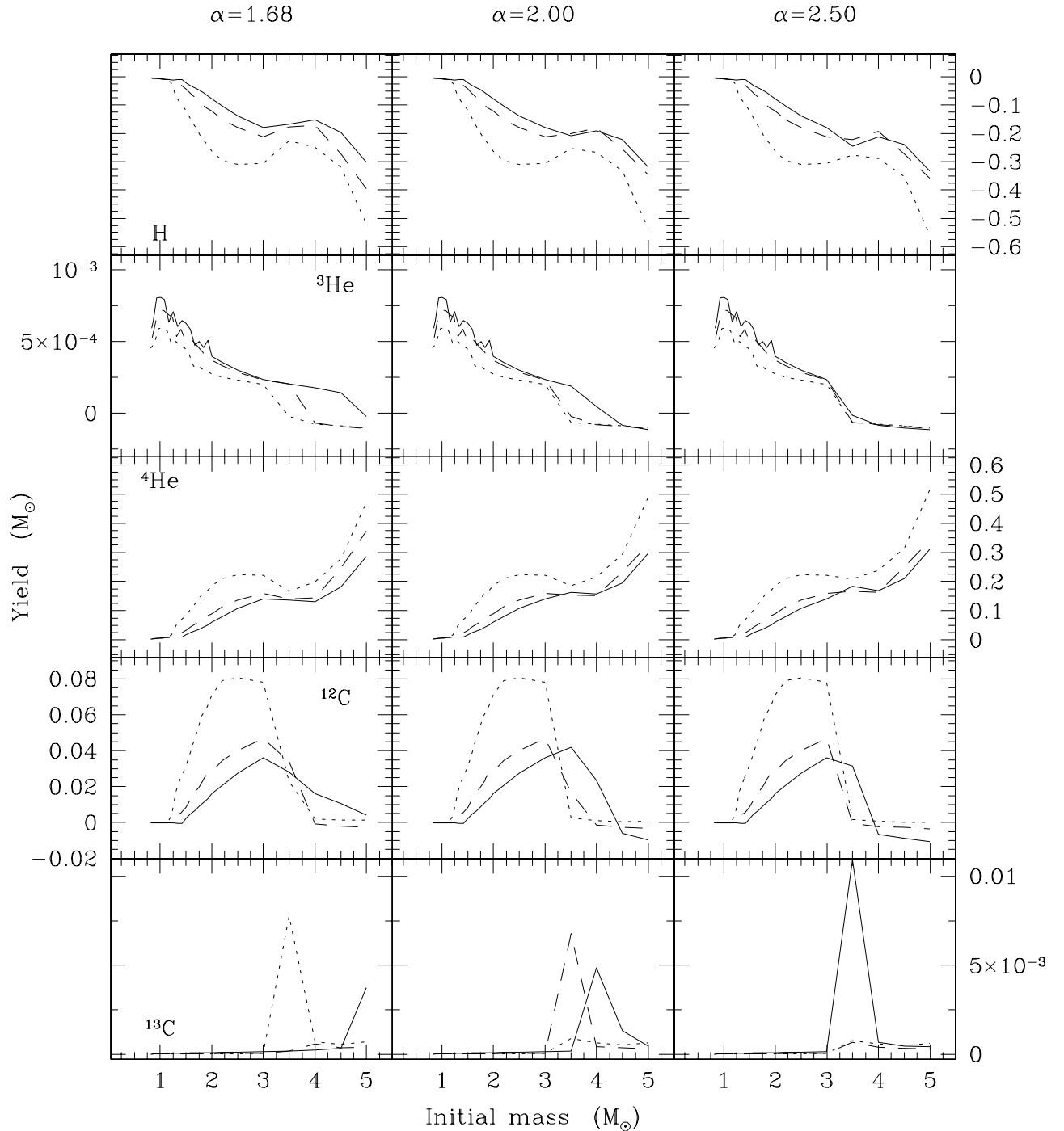
Fig. 1. Net yields M_y(k) (in M_\odot ) for each indicated chemical element (H, ^3\text{He} , ^4\text{He} , ^{12}\text{C} , and ^{13}\text{C} ) as a function of the initial mass (in M_\odot ) of the star. The solid, dashed, and dotted lines correspond to the metallicity sets Z = 0.019 , Z = 0.008 , and Z = 0.004 , respectively. Panels along each column refer to the same value of the mixing-length parameter
