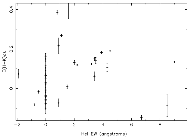
Fig. 7. Circumstellar excess versus Hel\ 2.058\ \mu m EW/\text{\AA}
