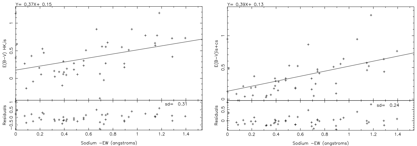
Fig. 3. (Left panel) a plot of E(B - V)_{(H-K)_{is}} , the IR (H - K) interstellar reddening, converted to an optical (B - V) colour versus sodium EW (Å). (Right Panel) a plot of (B - V)_{is+cs} versus the Na D_2 5890 Å line EW . The fitted lines are least squares fits minimised in the ordinate axis
