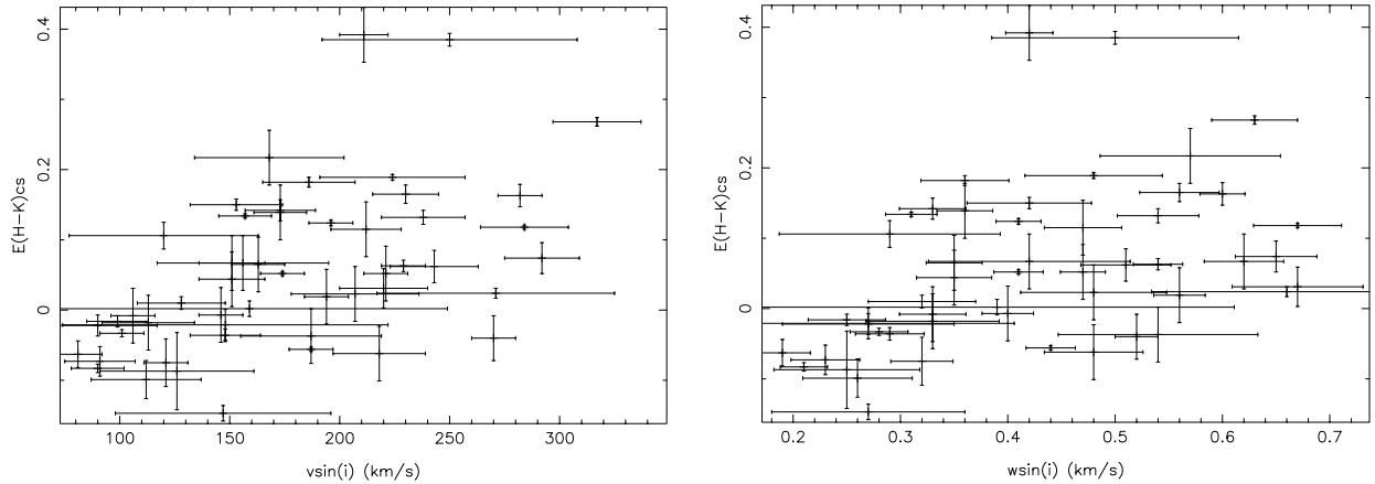
Fig. 9. Circumstellar excess versus v \sin(i) (left panel) and \omega \sin(i) (right panel)
