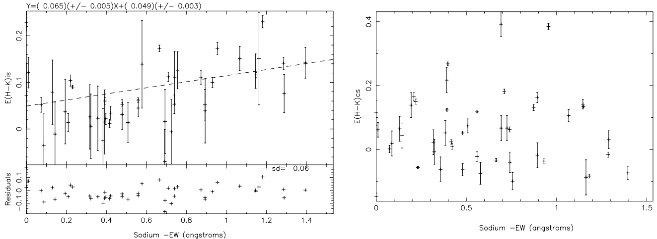
Fig. 2. Interstellar extinction versus Na D_2 5890 Å line EW (left panel), where the fitted line is a least squares fit weighted to the ordinate axis errors, and versus circumstellar excess (right panel). Note that as expected no correlation between the interstellar Na EW and the circumstellar excess is present
