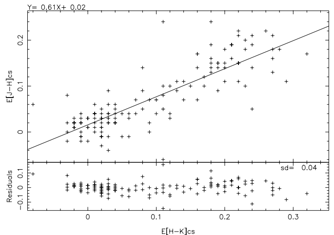
Fig. 1. Data extracted from Dougherty et al. (1994). The ratio \beta was calculated by means of a least squares fit, shown above as a solid line. Note that “sd” is the rms deviation of the residuals about the fitted line in the ordinate axis
