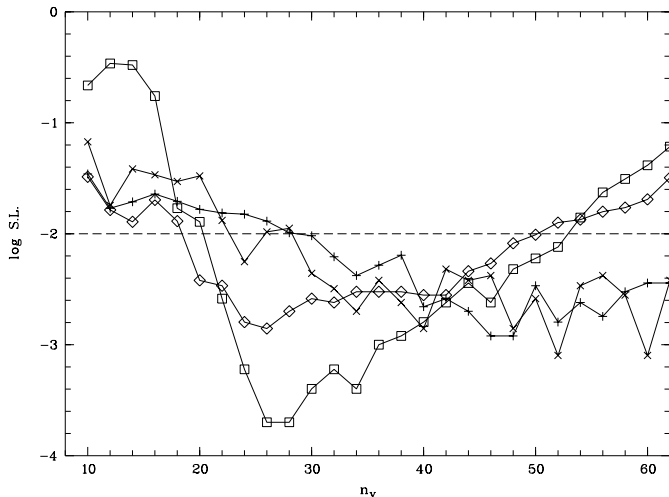
Fig. 2. The logarithmic significance level (S.L.) of the four statistical tests defined in Paper I, S with \Delta\theta_c = 60^\circ ( \square ), S_D ( \diamond ), Z_c^m ( + ), Z_c ( \times ), when applied to the new sample of 213 polarized quasars. n_v is the number of nearest neighbours around each quasar; it is involved in the calculation of averaged quantities. The dashed horizontal line indicates the 1% significance level
