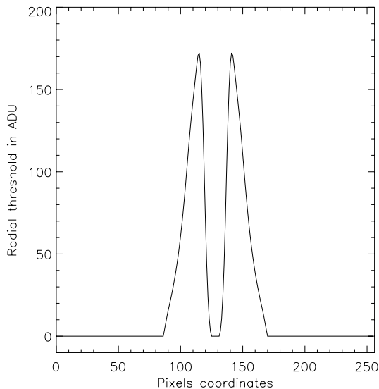
Fig. 1. An example of radial threshold obtained for the star HD 222493. A mask is used to select the region of interest: pixel 86 to 170
