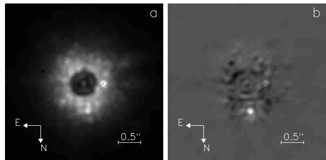
Fig. 9. Coronagraphic image of HD 184713 using long exposures a ) and the subtraction map b ) where the companion is clearly evidenced with its first bright Airy ring
