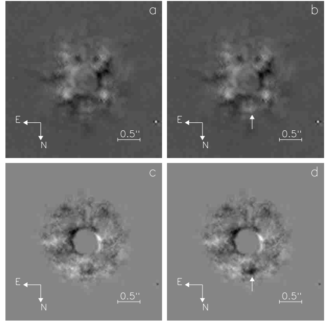
Fig. 6. Coronagraphic subtracted images of HD 192876 for direct integration of frames a,b ) and with a dark-speckle analysis c,d ). A faint companion ( \Delta m_k = 6 , arrow) is added to the map b,d ) to assess the detection threshold. The SNR is 1.8 with a direct integration and improves to 4.8 owing to the dark-speckle process
