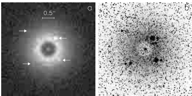
Fig. 2. Coronagraphic simulation of 200 frames each lasting 60 ms. Four companions (arrows) 5, 6, 7 and 8 magnitudes fainter than the star were added to the frames. The direct integration of frames is shown in a ) and b ) is the result obtained with a dark-speckle process on the same data cube (threshold: 10 ADU). Angular separation of the companions scaled to the resolution of a 3.6 m telescope at 2.2 \mu\text{m} are respectively 0.55'' , 0.65'' , 0.87'' , 1.09''
