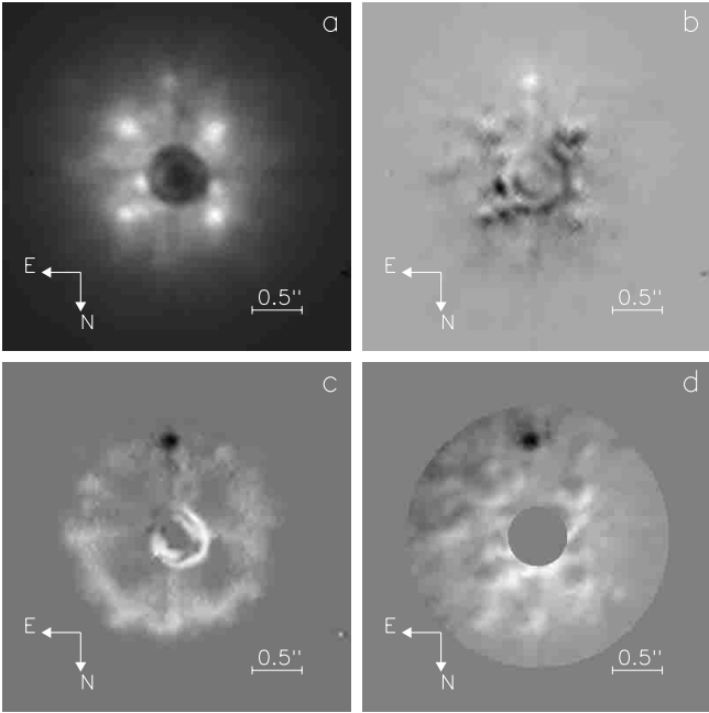
Fig. 3. Coronagraphic images of the binary star HD 222493 obtained with 600 frames lasting 60 ms each and a 0.63'' mask. The companion is already visible on the direct integration of frames a ) and is enhanced on the subtraction map b ). Lower images c ), d ) show the subtraction result using dark-speckle process with a constant threshold of 100 ADU c ) and a radial threshold d ), see Sect. 4. The companion now appears as a dark feature with an improved SNR
