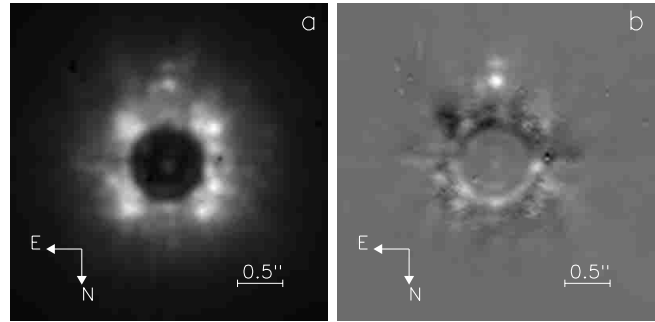
Fig. 4. Images of HD 222493 a ) obtained under good seeing conditions and long exposures ( 18 \times 2 s). The first companion's Airy ring is detectable on the subtraction frame b )
