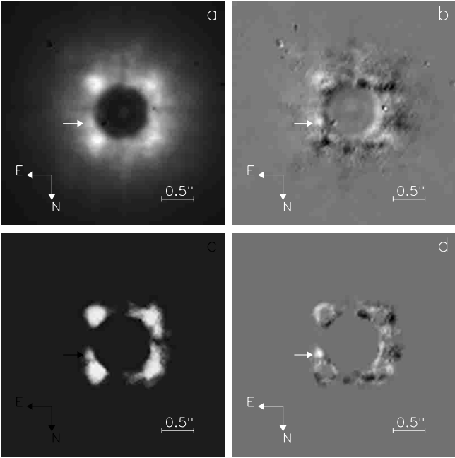
Fig. 7. Coronagraphic images of \eta Psc a ) and the result of reference star subtraction b ). Lower images show the dark-speckle process for the star alone c ) and the subtraction d ). The suspected companion is indicated by an arrow
