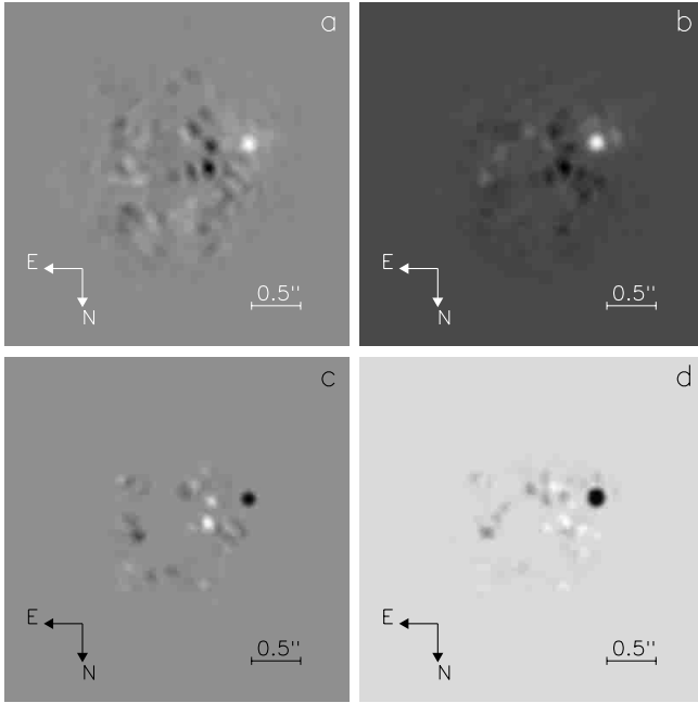
Fig. 5. Subtracted maps of the star \alpha Oph with direct integration of frames in two different atmospheric conditions a,b ) and processed with a dark-speckle analysis c,d )
