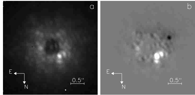
Fig. 8. Coronagraphic images of \nu Oph, displayed with a 0.5 power a ). The subtraction with \alpha Oph is also shown b ). The companion of \alpha Oph is visible as a dark feature
