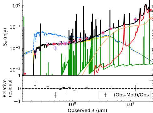
Best model for 2703664071644731101 ( z=1.36 , M_{\star}=10.47\pm0.24 , reduced \chi^2=0.66 )
