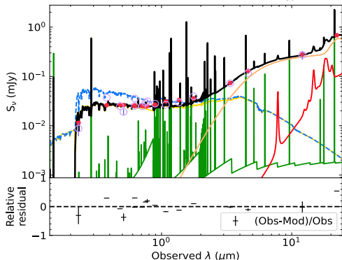
Best model for 2663093395657204902 ( z=1.37 , M_{\star}=10.12\pm0.62 , reduced \chi^2=2.3 )
