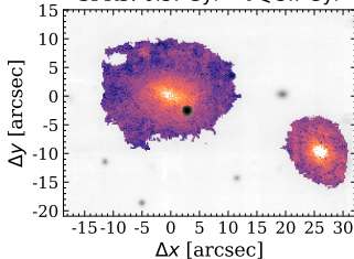
SFR3: 0.57 \text{ Gyr} < t \leq 5.7 \text{ Gyr}
