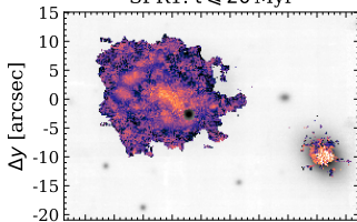
SFR1: t \leq 20 Myr
