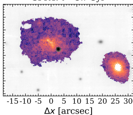
SFR4: t > 5.7 \text{ Gyr}
