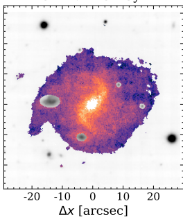
SFR4: t > 5.7 \text{ Gyr}
