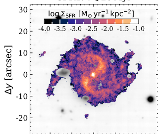
SFR3: 0.57 \text{ Gyr} < t \leq 5.7 \text{ Gyr}
