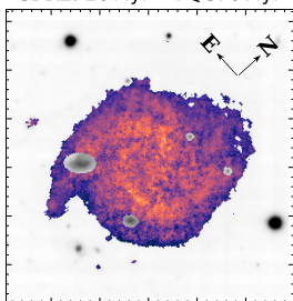
SFR4: t > 5.7 \text{ Gyr}
