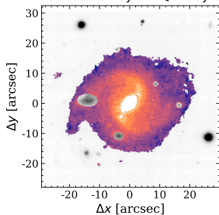
SFR3: 0.57 \text{ Gyr} < t \leq 5.7 \text{ Gyr}
