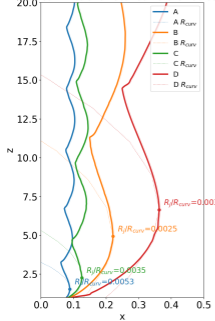
Streamlines and Local Curvature Radius
