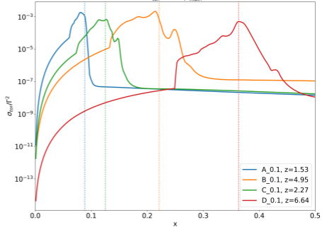
\sigma_{curv}/\Gamma^2 at z(x_{max})
