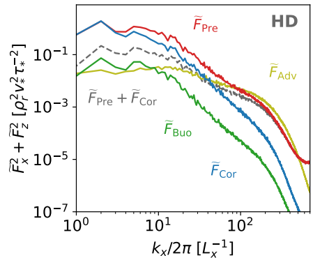
(c) Power spectra ( Co_* = 20 )
