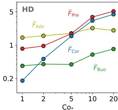
(b) RMS forces (y-averaged)
