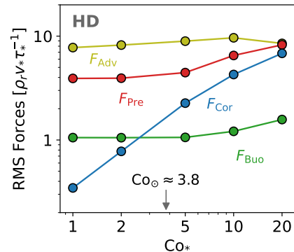
(a) RMS forces
