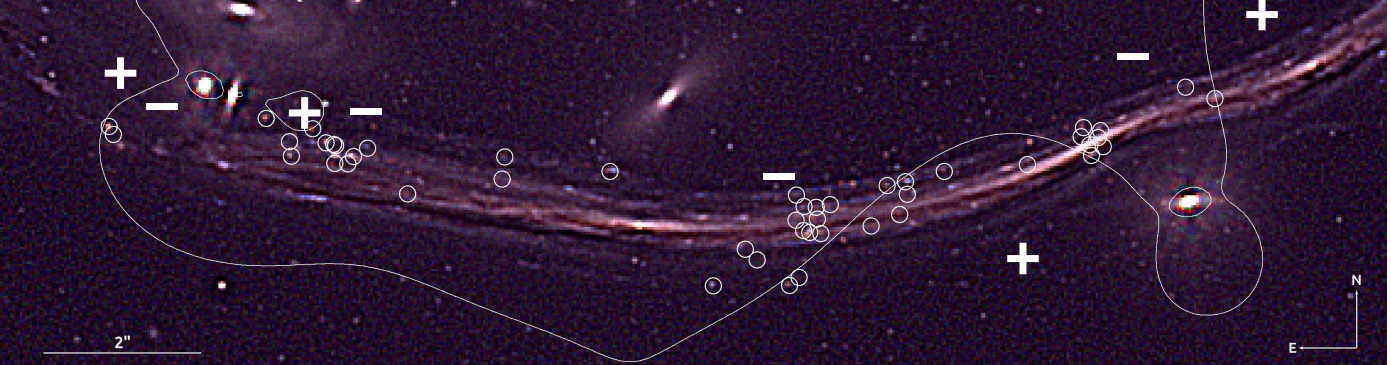
f115w+f150w+f200w (0.1")
