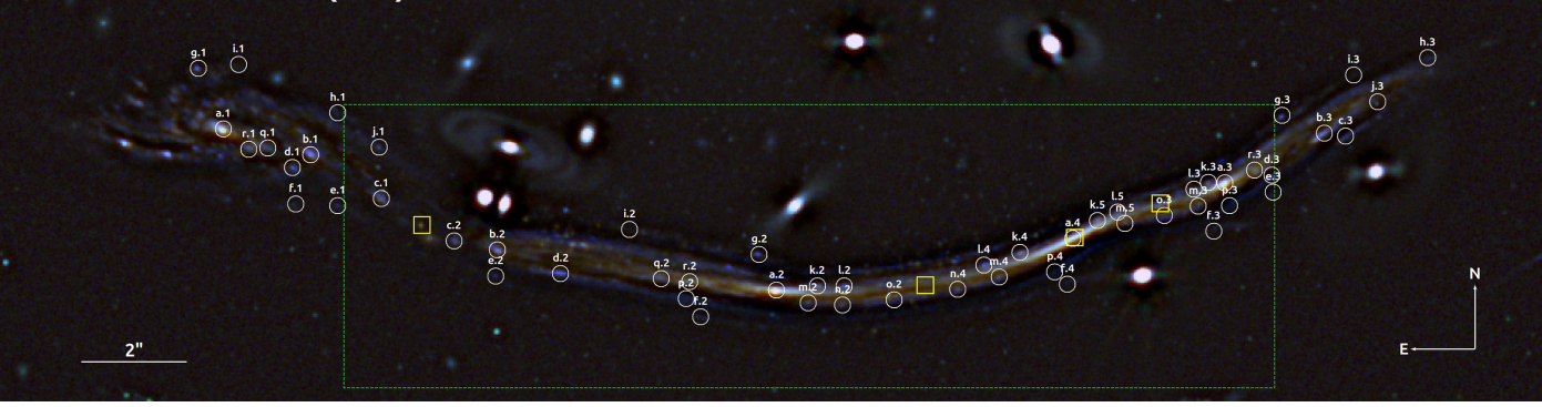
f090w+f200w+f356w (0.3")
