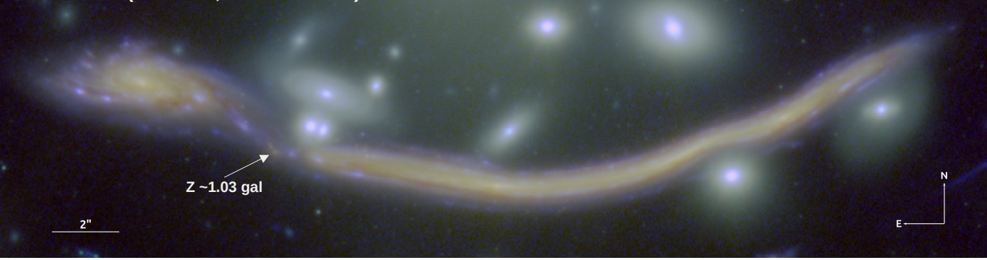
HST+JWST (16 filters, 0.2 - 5 micron)
