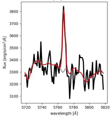
[NII] \lambda 5755
