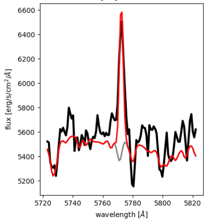
[NII] \lambda 5755
