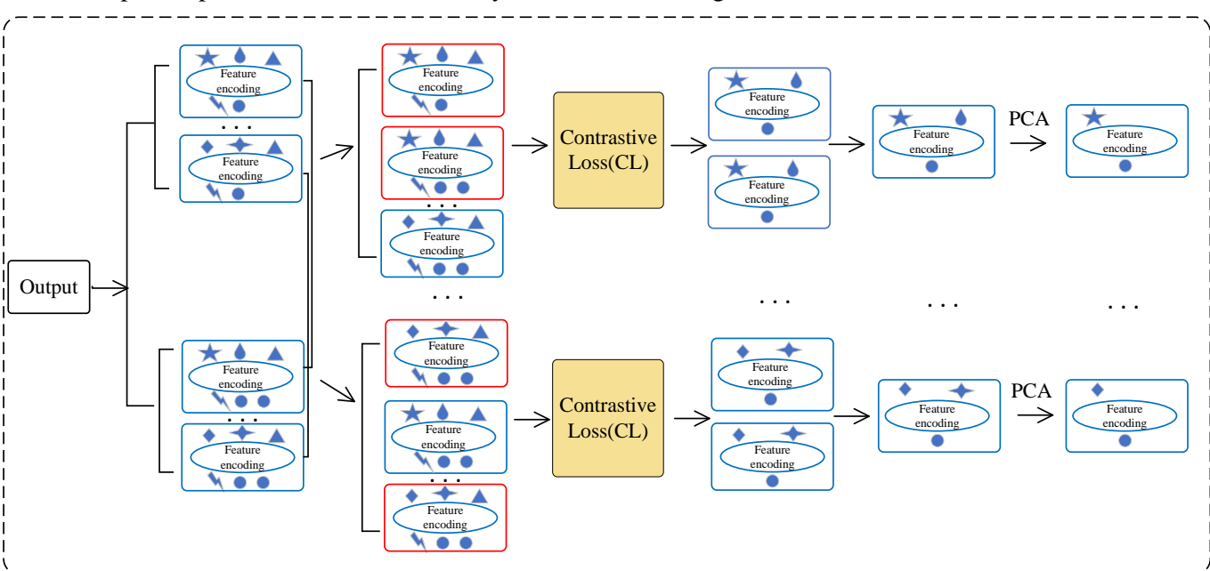
Step 2: Important feature extraction by contrastive learning and PCA
