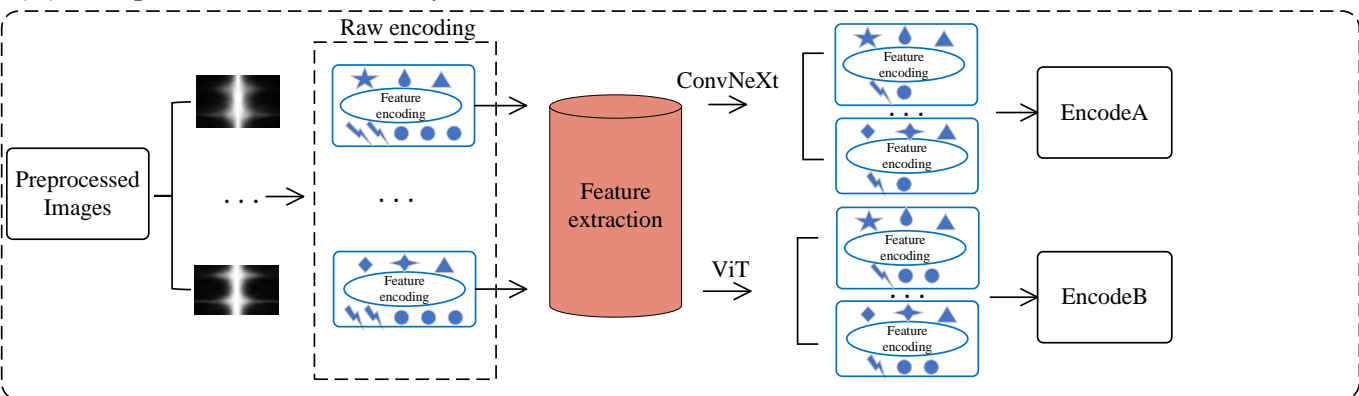
Step 2: Important feature extraction by contrastive learning and PCA
