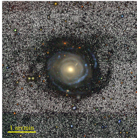
DECaLS
