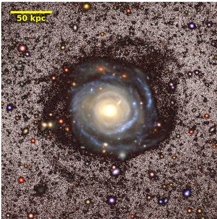
Malin 2 \log(M_*/M_\odot) = 11.3
