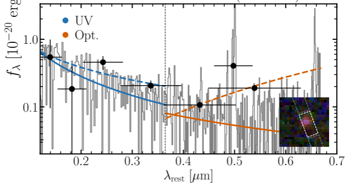
RUBIES-UDS-934230 ( z = 7.24 )
