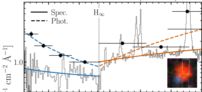
RUBIES-UDS-934230 ( z = 7.24 )
