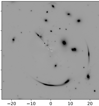
BCG subtracted
