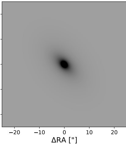
BCG model
