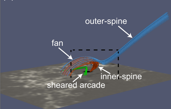
(a) NLFFF 14:36:00 UT
