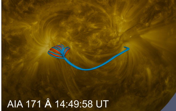
(f) Spherical NLFFF
