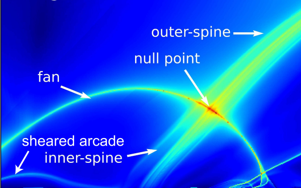
(c) \log_{10} Q
