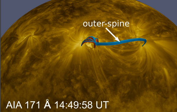
(e) Spherical NLFFF
