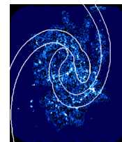
NGC 2835
