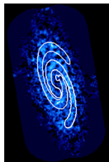
NGC 2090
