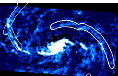
NGC 1672
