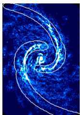
NGC 1566
