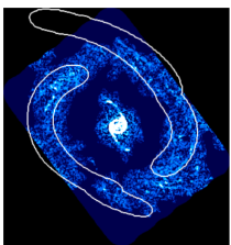
NGC 1512
