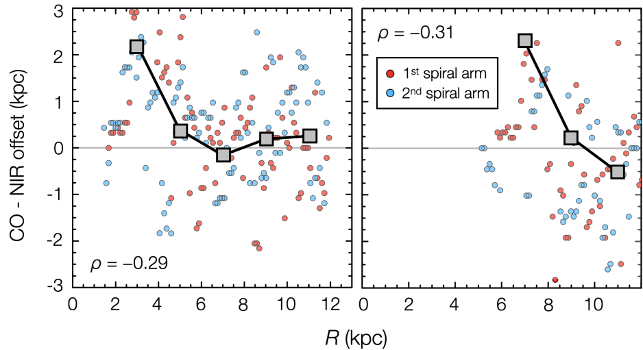
NGC 1566
