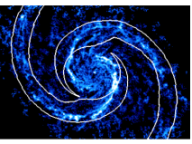
NGC 5194
