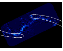
NGC 4731
