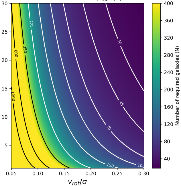
Minimum N for fixed ( v_{\text{rot}}/\sigma, \varepsilon )
