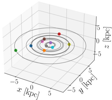
Face-on disk
