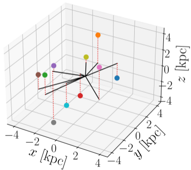
Spherical
