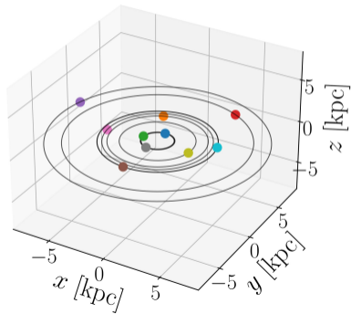
Edge-on disk
