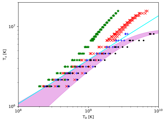
(b) B = 10^{12} G
