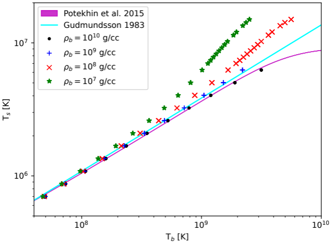
(a) B = 10^8 G
