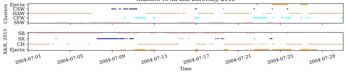
Clusters vs Xu and Borovsky, 2015
