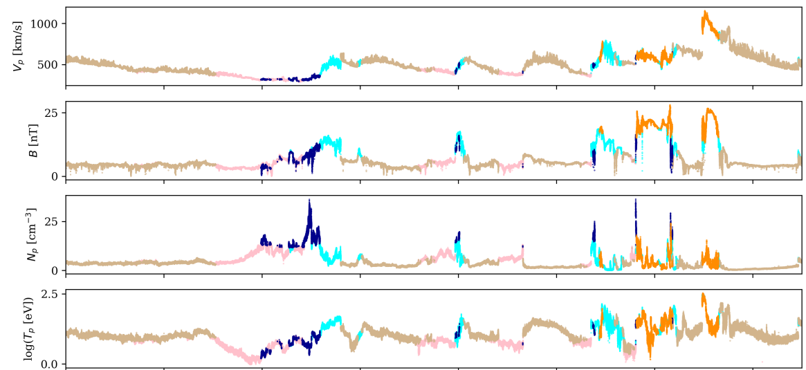
Clusters vs Xu and Borovsky, 2015
