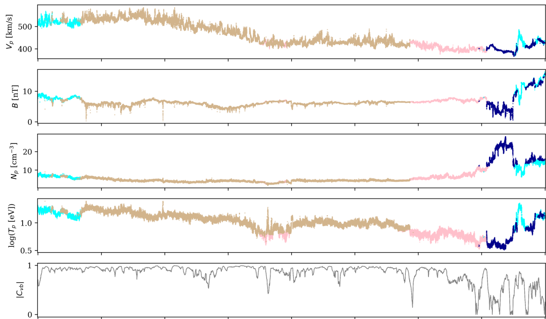
Clusters vs Xu and Borovsky, 2015
