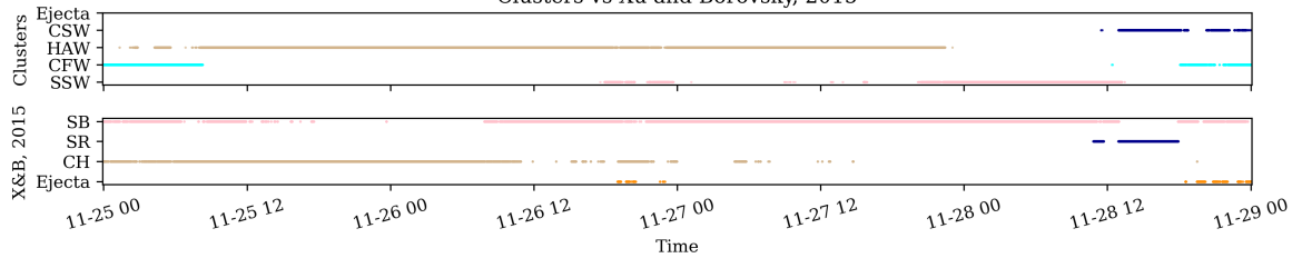
Clusters vs Xu and Borovsky, 2015
