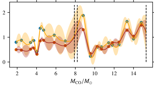
Z = Z_{\odot} , Case Bc
