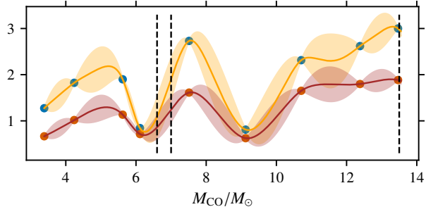
Z = Z_{\odot} , Case C
