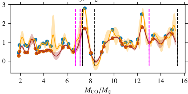
Z = Z_{\odot} , single & Case A
