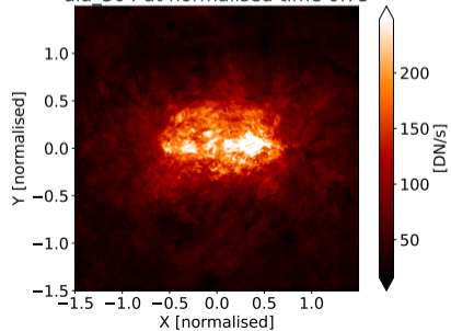
aia_304 at normalised time 0.75
