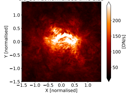
aia_304 at normalised time 1.25
