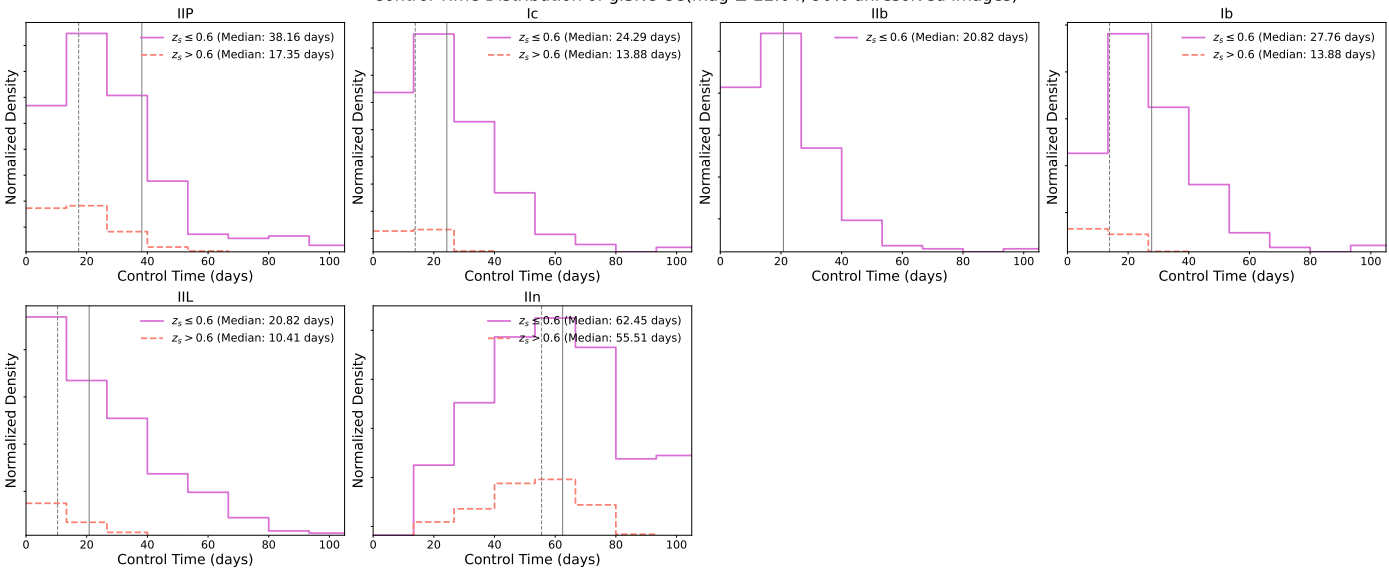
Control Time Distribution of gISNe CC(mag \leq 22.04, 90% unresolved images)
