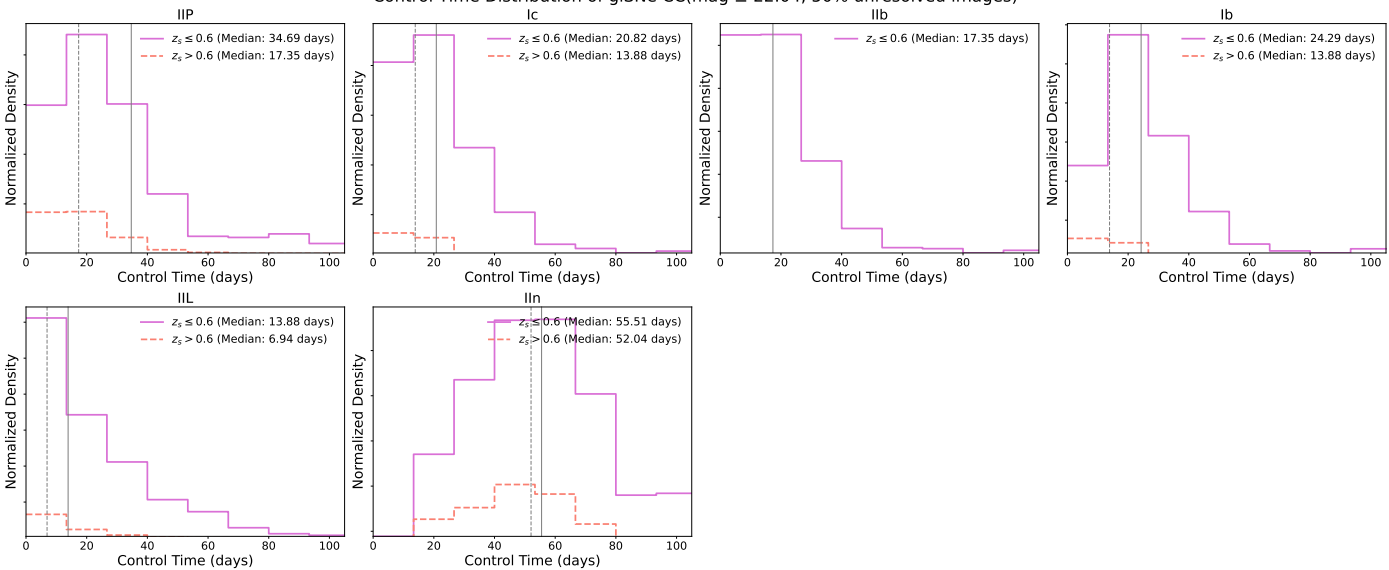
Control Time Distribution of gISNe CC(mag \leq 22.04, 50% unresolved images)
