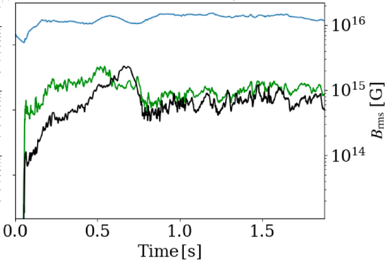
Strong initial B_{\phi}^{m=0}
