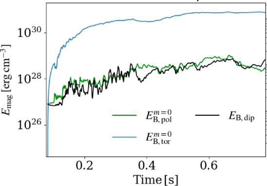
Weak initial B_{\phi}^{m=0}
