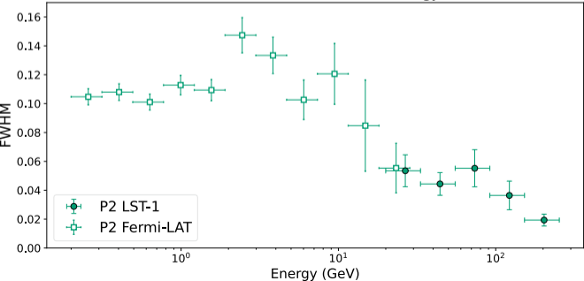
P2 FWHM vs Reconstructed Energy
