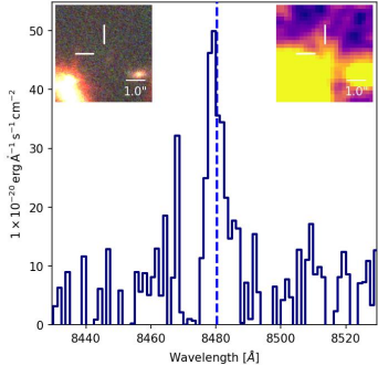
z = 5.9757 LyA 43.1c
