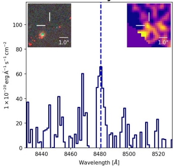
z = 5.9759 LyA 43.1d
