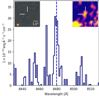
z = 5.9753 LyA 43.1b
