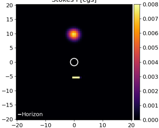
Stokes I [cgs]
