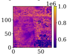
Temperature diagnostic Mg IX 706 / Mg VIII 772
