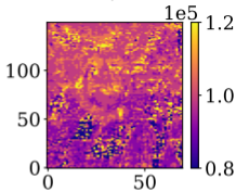
Temperature diagnostic O IV 787 / O III 703
