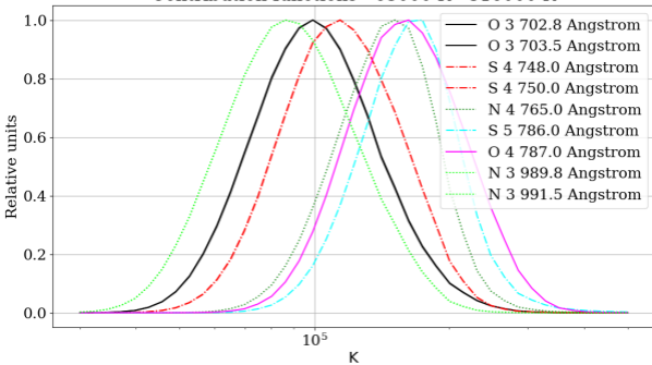
Contribution functions - 63000 K - 316000 K
