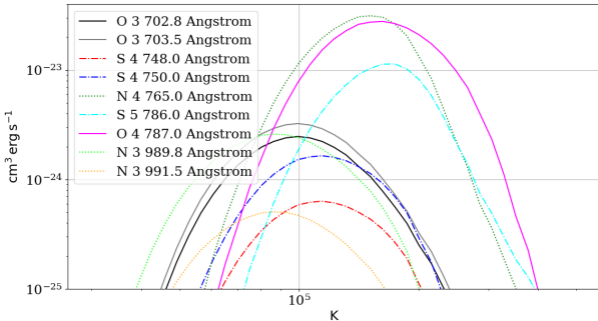
Contribution functions - 63000 K - 316000 K
