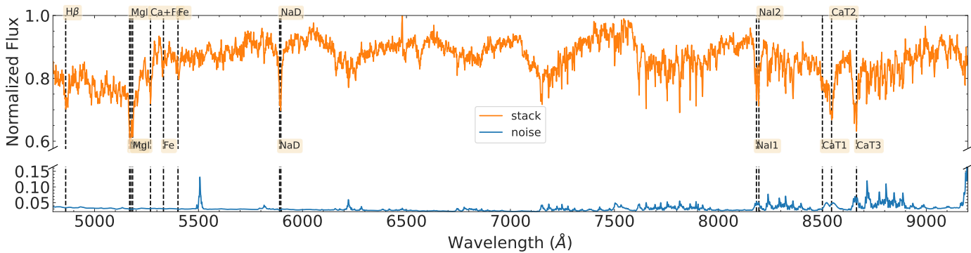
Stacked all GC spectra
