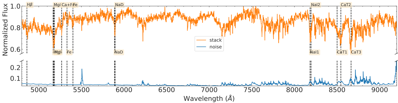
Stacked outer GC spectra
