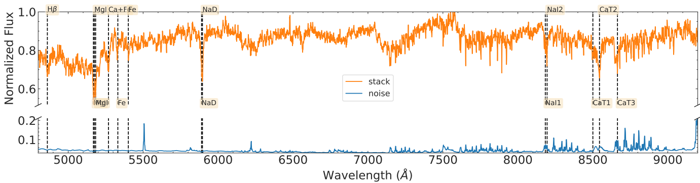
Stacked inner GC spectra
