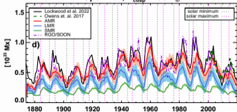
Open flux, R_{\text{cusp}}=1.50 R_{\odot}
