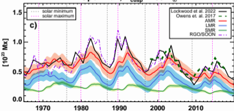
Open flux, R_{\text{cusp}}=1.50 R_{\odot}
