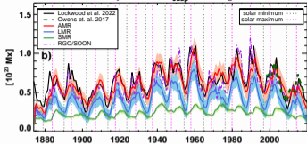
Open flux, R_{\text{cusp}}=1.40 R_{\odot}
