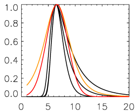
Gauss, Kappa, NIG
