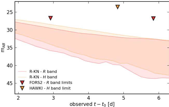
POSSIS Red KN lightcurves at z=0.64
