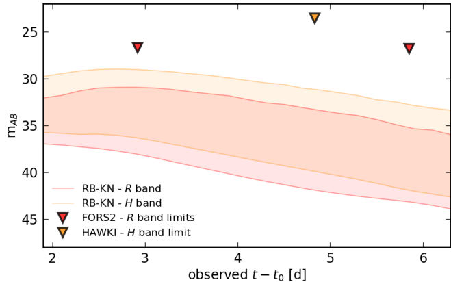
POSSIS Red+Blue KN lightcurves at z=0.64
