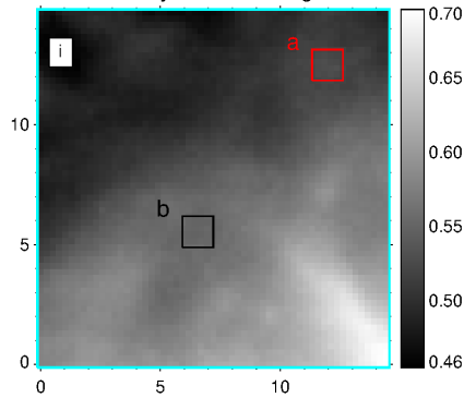
Time-Averaged Normalized Intensity in Bright Point
