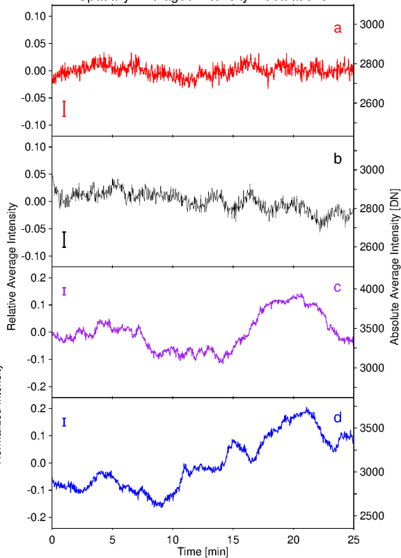
Spatially-Averaged Intensity Fluctuations
