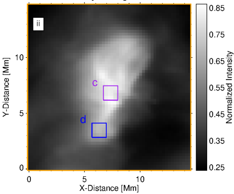
Time-Averaged Normalized Intensity in Bright Point
