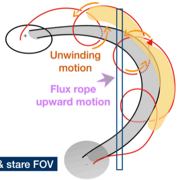
d) Filament material during the eruption
