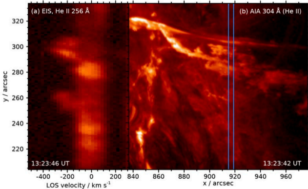
c) Filament material pre-eruption
