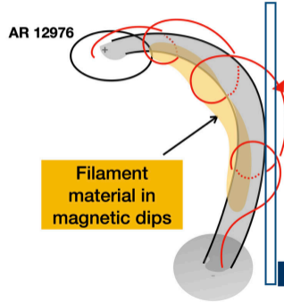
c) Filament material pre-eruption
