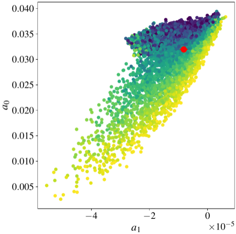
Basic reaction network
