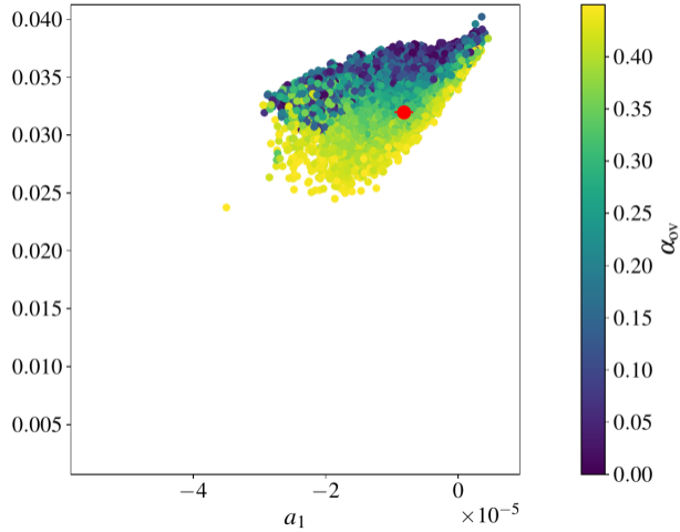
Full reaction network
