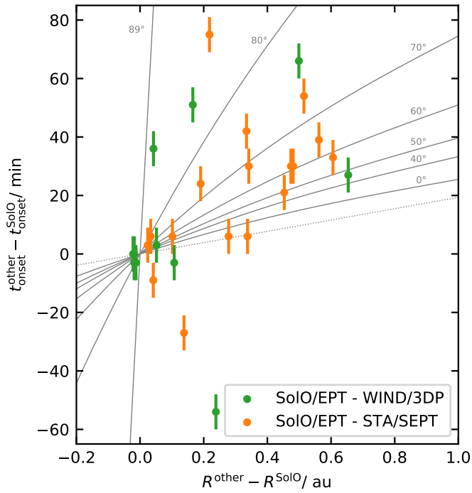
onset delay vs difference in radial distance
